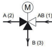
Diverting valve
