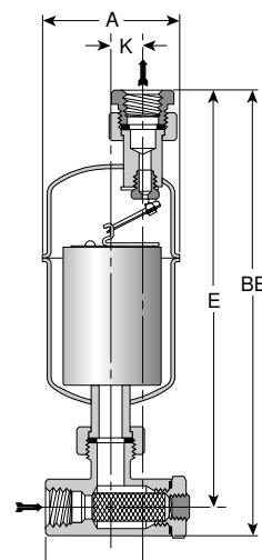
Figure 19-2. Series U-1010 Trap with strainer
