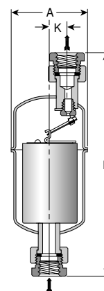
Figure 19-3. Series U-1010 Traps
