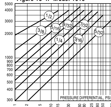
Figure 18-4. Model 1013
