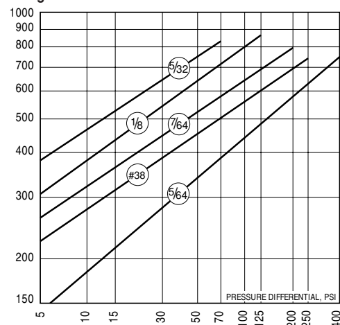
Figure 14-2. Model 2011
