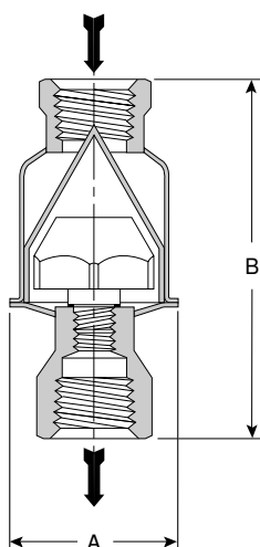
Figure 31-2. Model WT-1 Trap
