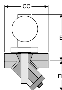
Figure 15-3. Model 2011 with 2010 IS Connector.
