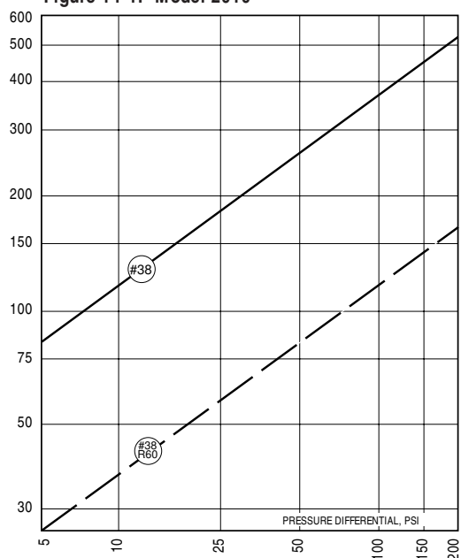
Figure 14-1. Model 2010
