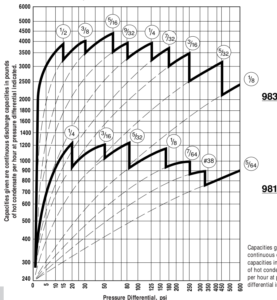
Chart 20-1. Series 980 Traps
