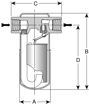
Figure 17-1. Model 1811 Trap
