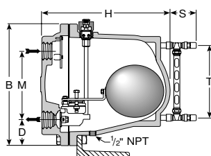
Figure 29-2. Series L and LS, F&T shown
