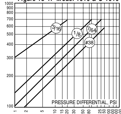
Figure 18-2. Model 1011 & U-1011
