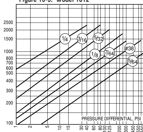
Figure 16-3. Model 1812
