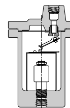
Figure 11-1. Series 300 - 400 Traps with internal check valve
