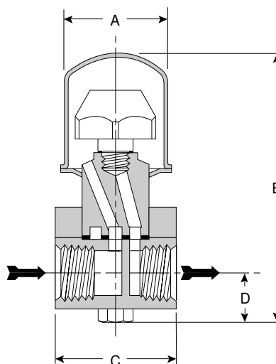
Figure 31-3. Model WT-2000 Trap
