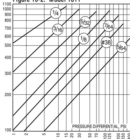
Figure 16-2. Model 1811
